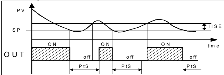
"Pts" example with "Func" = Cool
