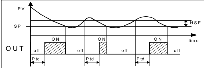
"Ptd" example with "Func" = Cool
