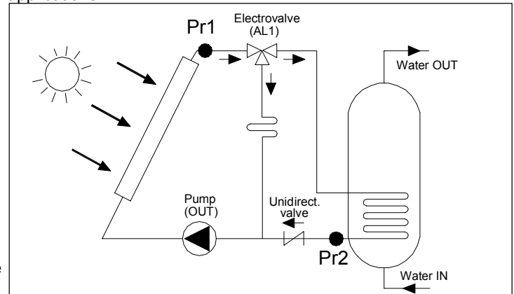
Case A – Minimum alarm on probe Pr1 (Anti-ice on the solar collector)
